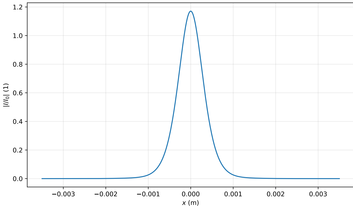
Intensity profile I(x, y = 0, z = 2.707m)/I_0 , P_{in}=0.8P_{cr} , artificial time
